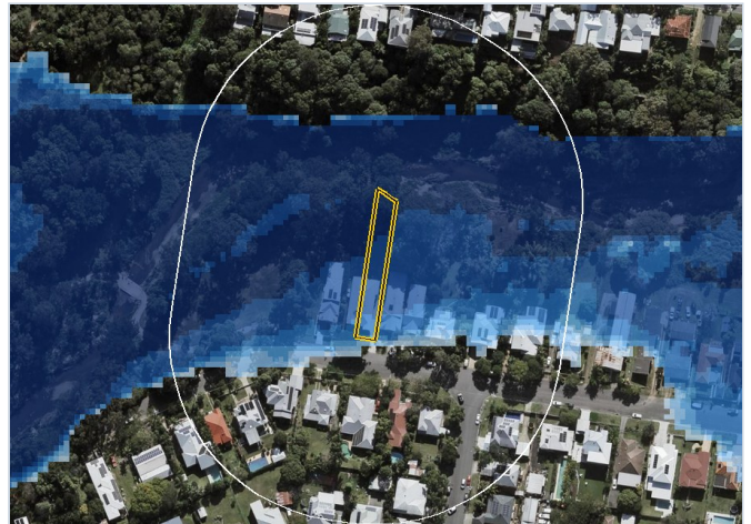
FIGURE 24. 50-YEAR ARI - ULTIMATE - FUTURE CLIMATE
