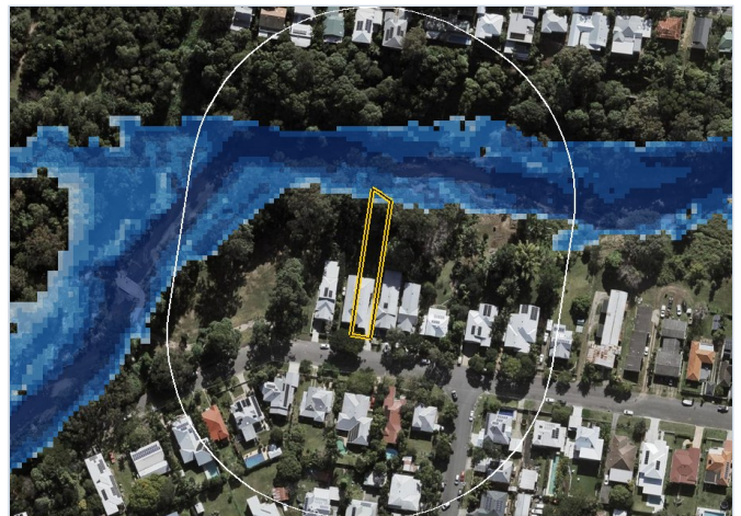
FIGURE 20. 2-YEAR ARI - ULTIMATE - FUTURE CLIMATE
