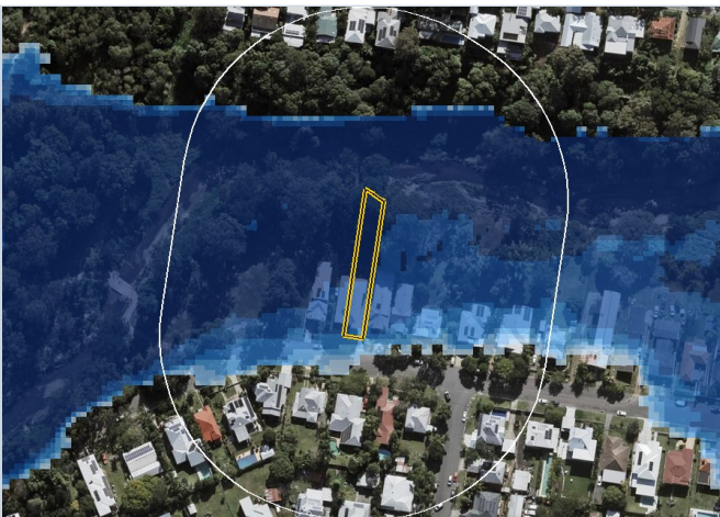
FIGURE 25. 100-YEAR ARI - ULTIMATE - FUTURE CLIMATE
