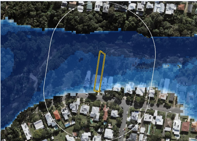
FIGURE 23. 20-YEAR ARI - ULTIMATE - FUTURE CLIMATE
