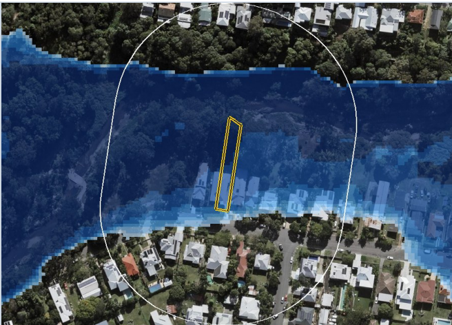
FIGURE 17. 200-YEAR ARI - FUTURE CLIMATE
